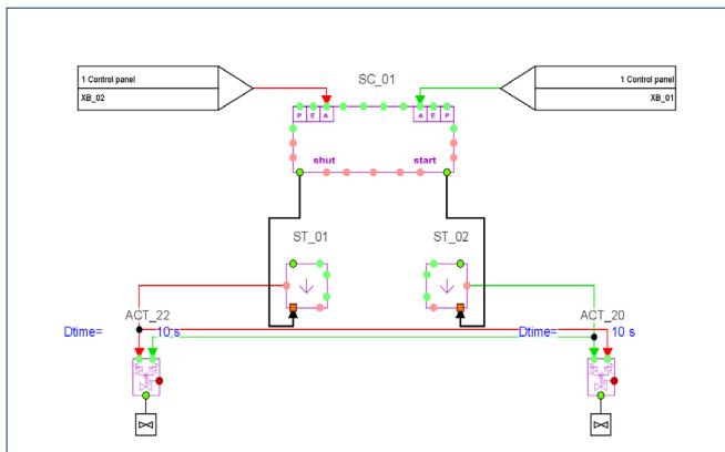
An example of a modelled sequence logic. Colour of the binary signal shows whether the value of the binary signal is true or false.
